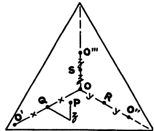
FIG. 3.—Template for cubic point-groups.
